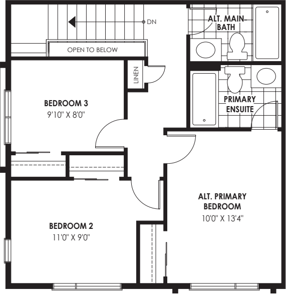
OPT. THIRD FLOOR PLAN ELEV. Flex Plan Option Available at Decor Centre
