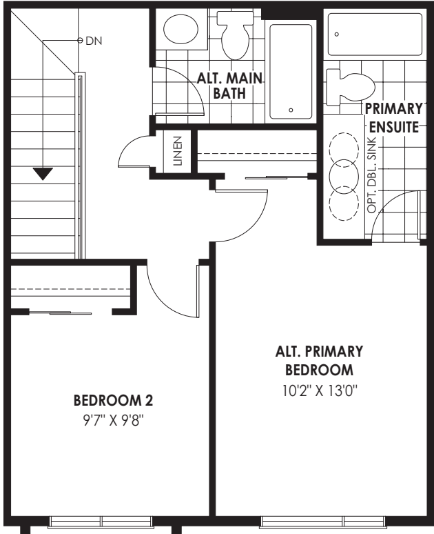
OPT. THIRD FLOOR PLAN ELEV. Flex Plan Option Available at Decor Centre
