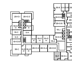
PODIUM LEVEL 8
