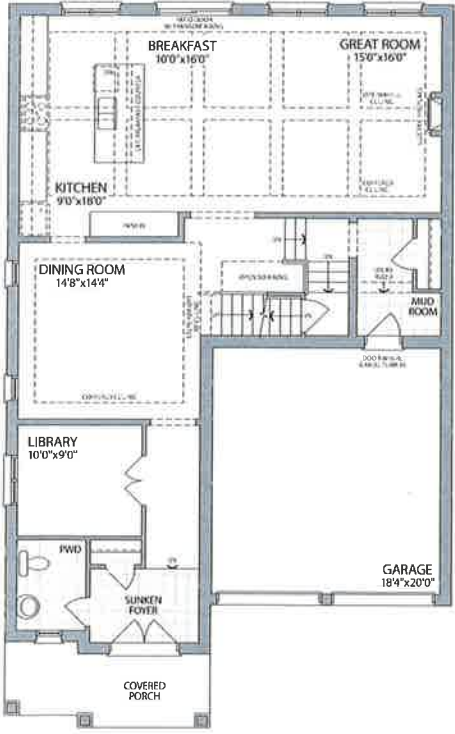
GROUND FLOOR ELEVATION 1
