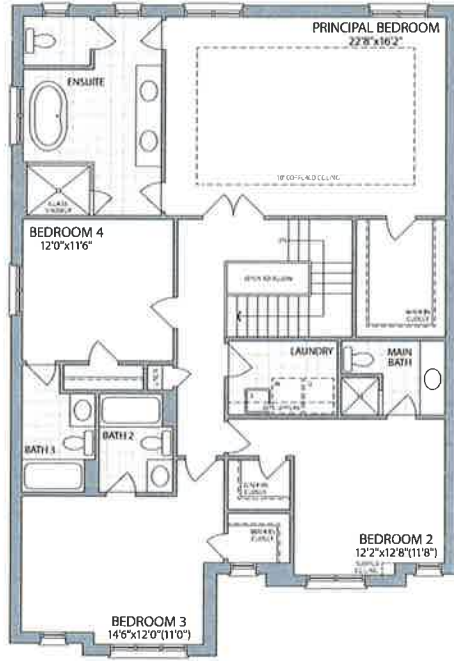
SECOND FLOOR ELEVATION 1
