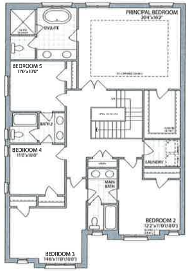
SECOND FLOOR W/OPT 5 BEDROOMS ELEVATION 1
