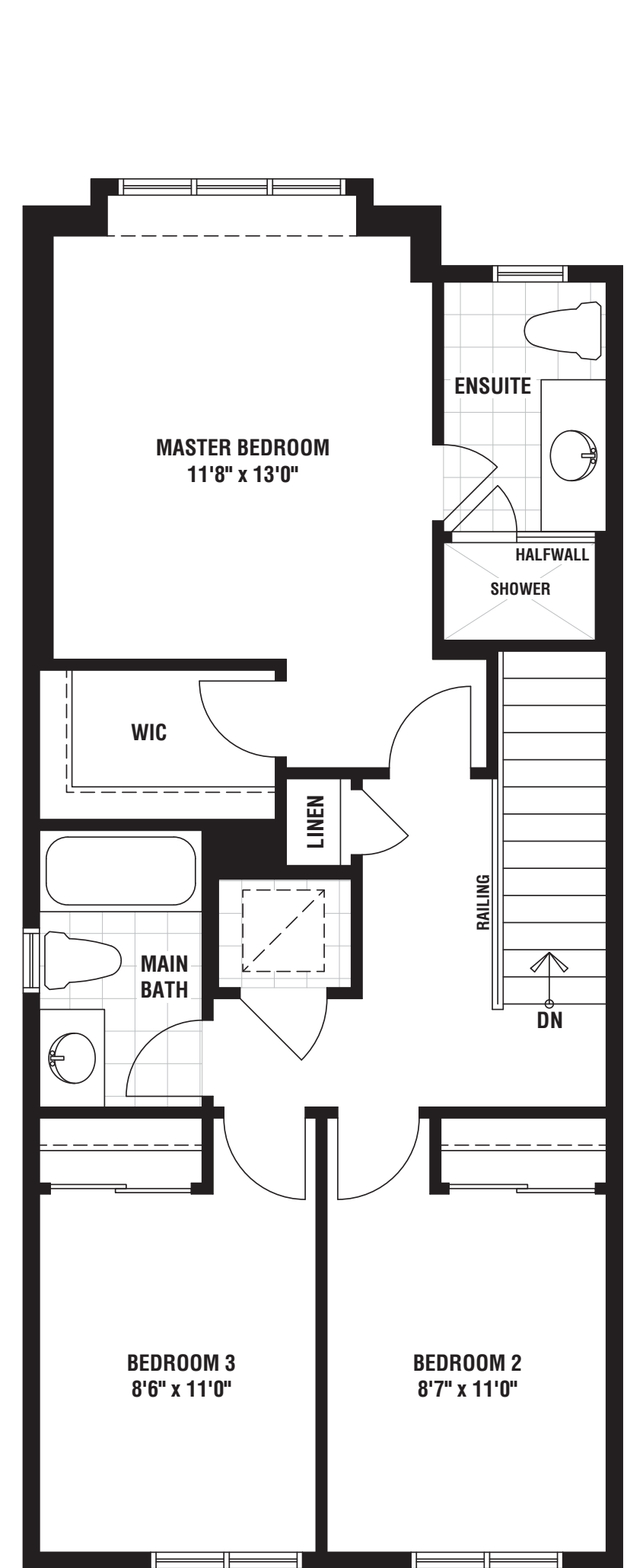
UPPER FLOOR PLAN ELEVATION 'A4'
