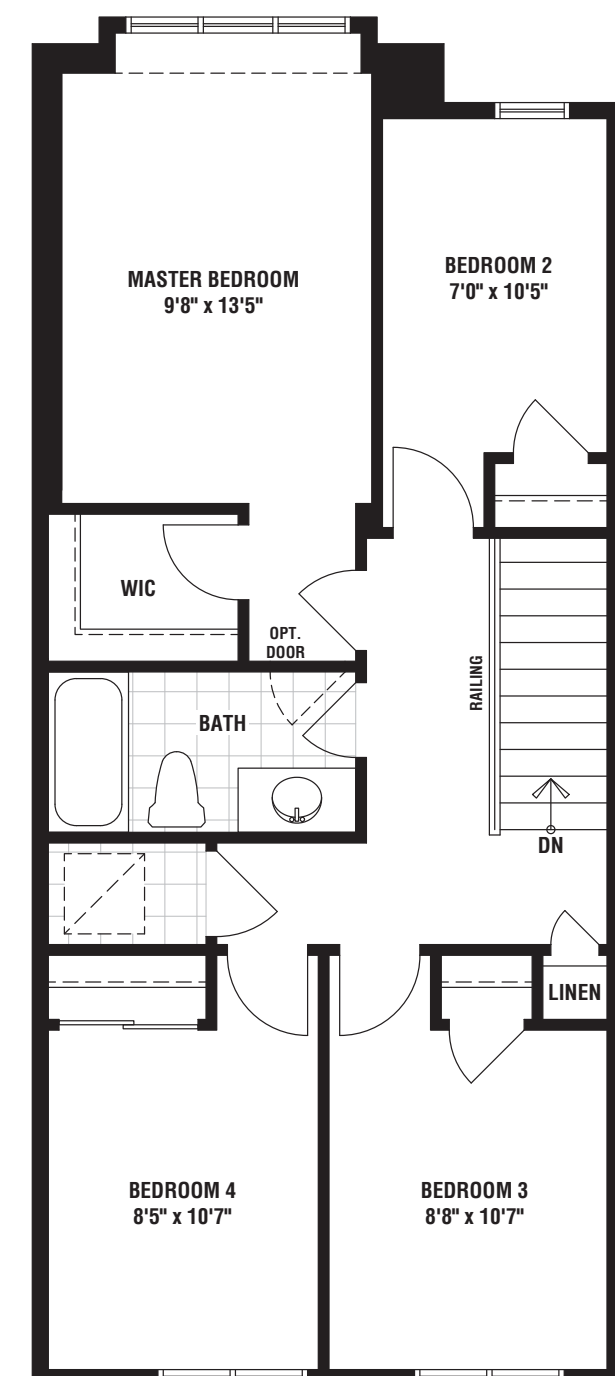
ALT. 4 BEDROOM UPPER FLOOR PLAN ELEVATION 'A4'
