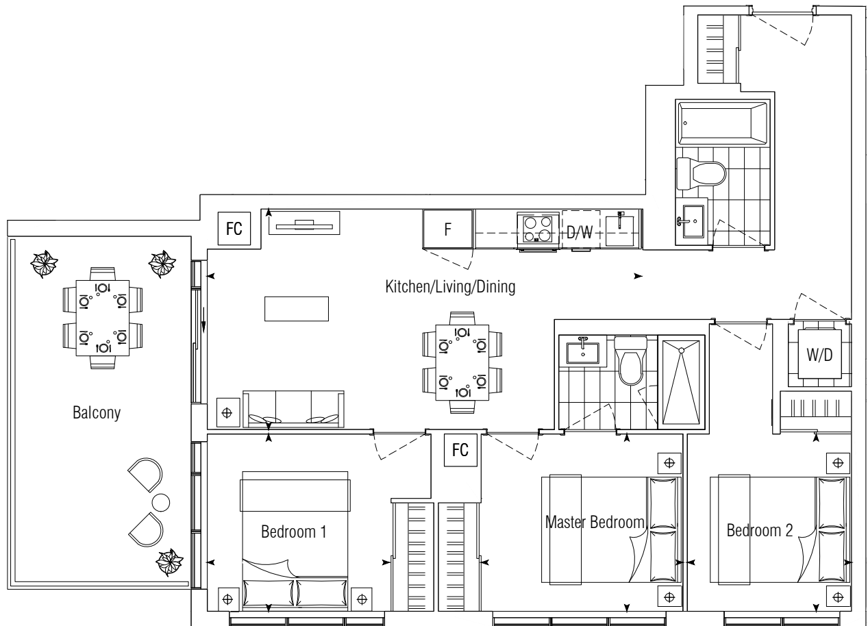
FLOORS 2-7
